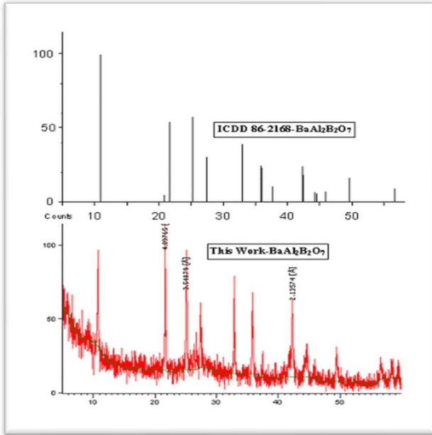
Fig. 1. XRD pattern obtained for \text{BaAl}_2\text{B}_2\text{O}_7:\text{Sm}^{3+} prepared by a solution combustion synthesis.
