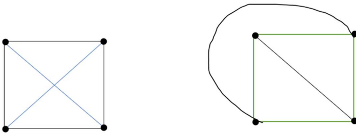
Planar graph
