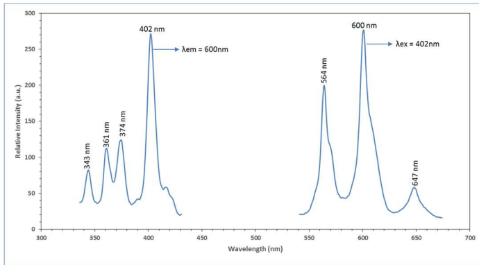
Fig. 2. Excitation & Emission Spectra of \text{Ba}_{(1-x)}\text{Al}_2\text{B}_2\text{O}_7:\text{Sm}^{3+} ( x = 0.02 mol) phosphor.
